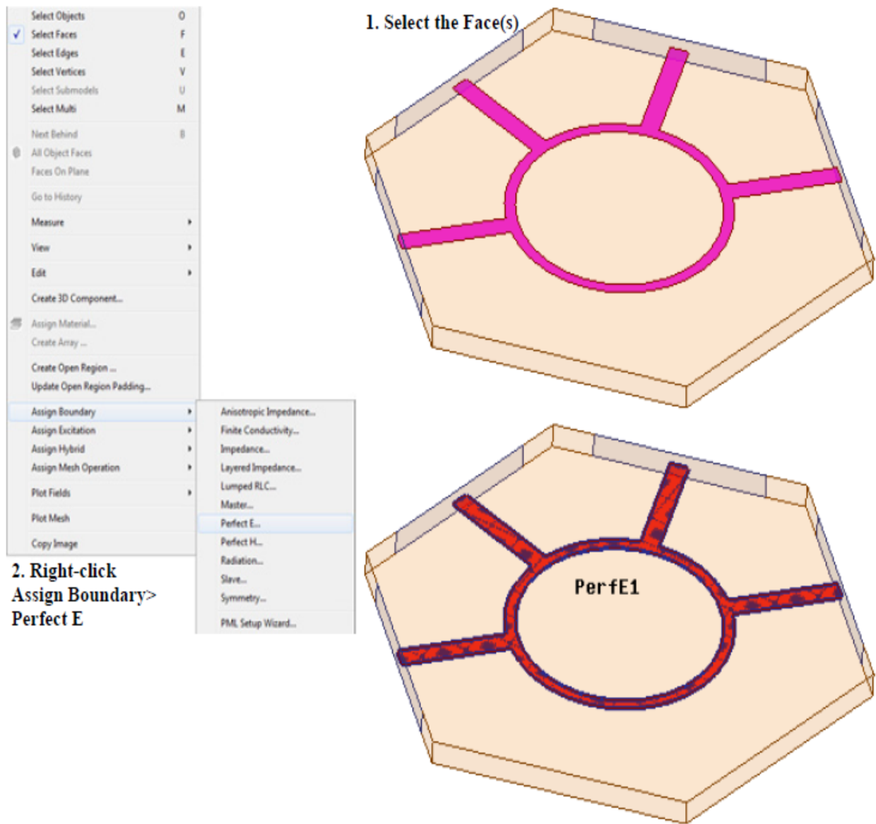
Figure 5-4 Perfect E Boundary assignment
