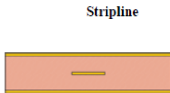
Figure: Port height is determined by ground plane spacing, and port touches both upper and lower ground planes.
